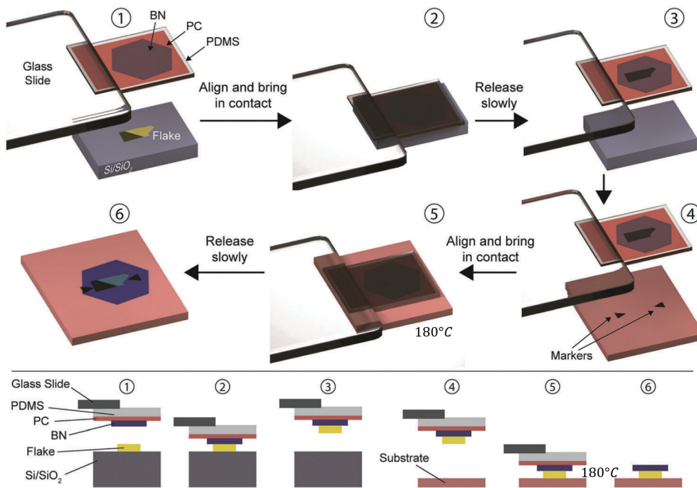
Figure 3.35 Van der Waals pick-up transfer method: The flake to be transferred is exfoliated onto a Si/SiO 2 substrate (1). A stack composed of PDMS with a layer of PC and a hBN flake is attached to a glass slide. The hBN is brought into contact with the target flake (2), and by releasing the contact slowly, the target flake can be picked up, remaining attached to the hBN flake (3). The stack is then positioned on top of the target substrate (4) and brought into contact (5). After melting the PC-film at 180°C, the target flake capped by the hBN flake can be transferred by slowly releasing the contact (6). Adapted from [79]
