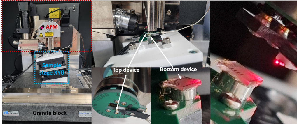
Figure 3.37 Images of the QTM setup.
