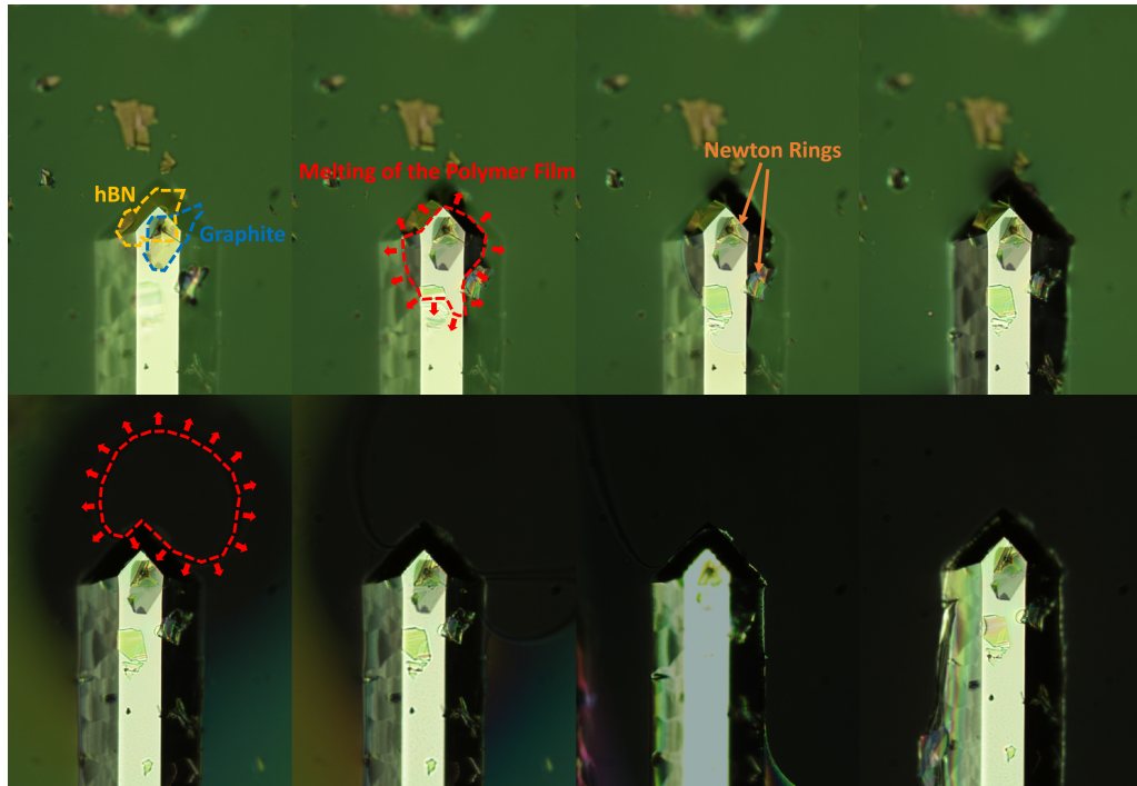
Figure 3.32 Top Row: Polymer film adheres on the heated cantilever ( 50^{\circ}\text{C} ) and melts. Bottom Row: After further heating ( 120^{\circ} ) film crumbles, leaving the cantilever detached from the transfer slide
