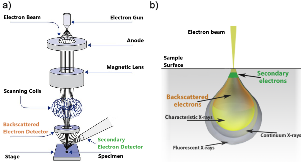
Figure 3.6 a) SEM setup. b) Schematic of electron beam interaction. Adapted from [62][63].
