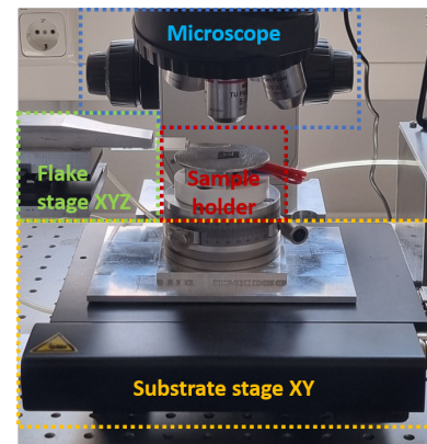
Figure 3.3 Transfer setup.
