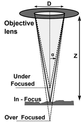
Figure 3.9 Beam geometry. Adapted from [68].
