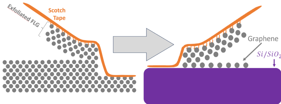
Figure 3.2 Scheme of two representative steps of mechanical exfoliation. On the left, Scotch tape is used to exfoliate FLG from bulk graphite, and on the right, the same Scotch tape is pressed against a silicon chip (in purple), resulting in a layer of graphene being deposited. Adapted from [58].
