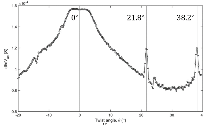
Figure 4.16 Measured conductance, \frac{dI}{dV} , versus rotation angle \theta between two graphite flakes in direct contact ( V_b = 0.1V , T = 300K ). The sample and tip remain in continuous contact throughout the measurement. Commensurate angles 0^\circ , 21.8^\circ , and 38.2^\circ are indicated by vertical lines.
