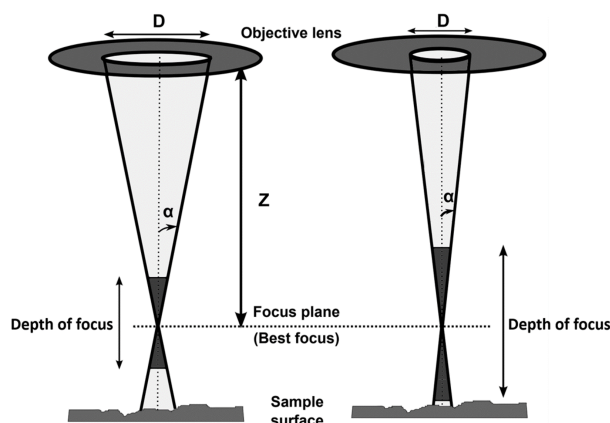
Figure 3.18 Relationship between the aperture diameter and depth of focus. Adapted from [68].
