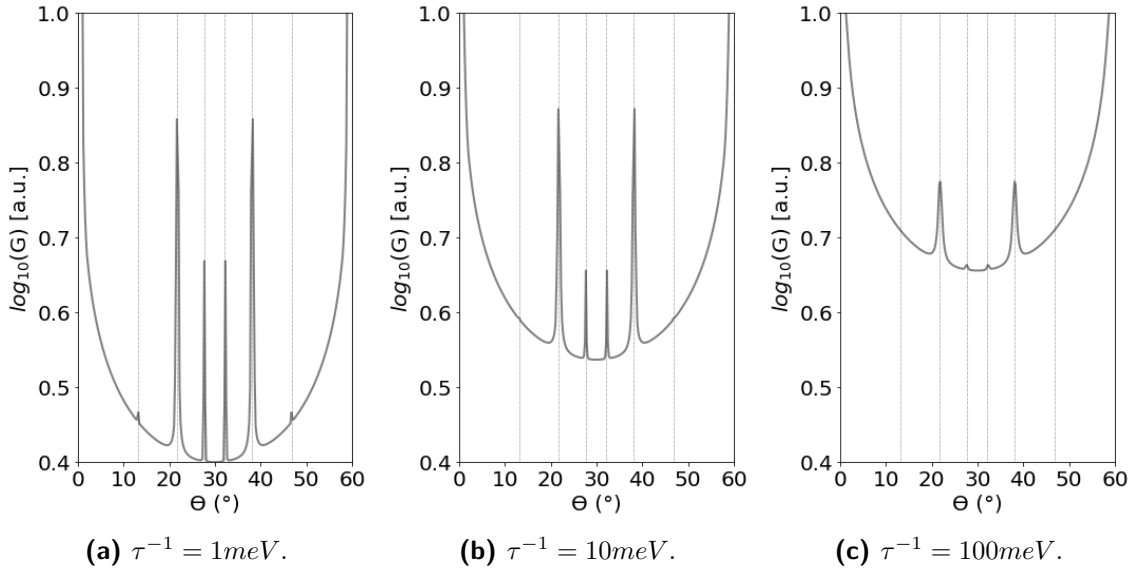
Figure 4.10 Simulated interlayer conductance G as a function of twist angle \theta and E_F = 0.1eV . The eight conductance peaks correspond to the commensurate angles near 0^\circ , 13.2^\circ , 21.8^\circ , 27.8^\circ , 32.2^\circ , 38.2^\circ , 46.8^\circ , and 60^\circ .
