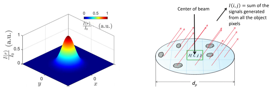
Figure 3.8 Finite probe size. Adapted from [67][64]
