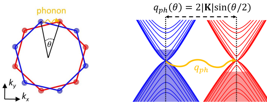
Figure 4.17 Fermi surfaces in k -space of the top and bottom graphite layers (left) and the corresponding energy bands (right). At a finite twist angle, there is a momentum mismatch between these energy bands, and momentum-conserving electronic tunneling between the layers can occur only via the emission or absorption of a phonon that provides the missing momentum q_{ph}(\theta) . Adapted from [92].
