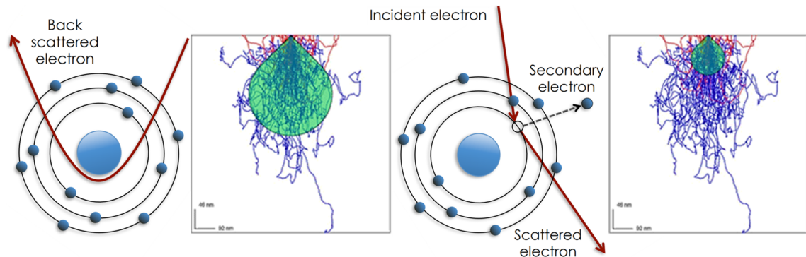
Figure 3.10 Electron-trajectory simulations. Blue (red) trajectories mark BSEs (SEs). Green area defines the interaction volume and origin of BSEs (left) and SEs (right). Adapted from [70][71].
