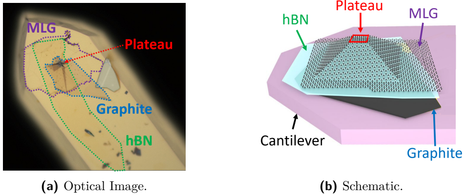
Figure 3.34 Tip device. Adapted from [14].
