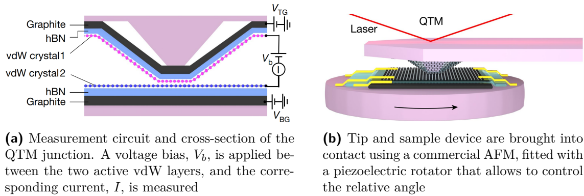
Figure 3.38 Schematic of the QTM setup. Adapted from [14].
