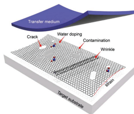
Figure 5.3 Schematic illustration of the as-transferred graphene film on target substrates with the assistance of transfer medium, highlighting the issues of cracks, unintentional doping, contamination, wrinkles, and strains. Adapted from [104]
