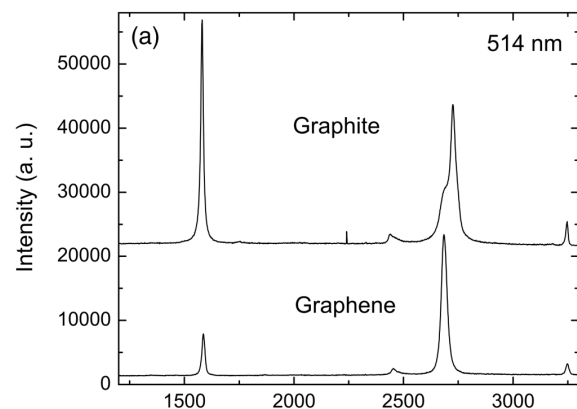
(b) Raman spectrum of graphene and graphite.
