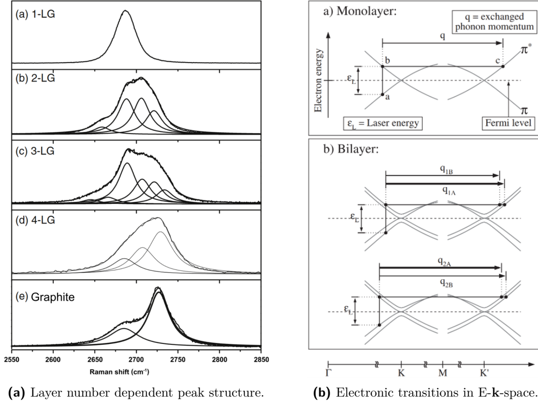
Figure 3.5 The 2D peak in FLG systems. Adapted from [61][60].
