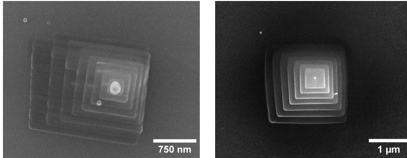
Figure 3.21 Typical observed spatial shift of deposited layers before(left) and after(right) modification of the preparation process.
