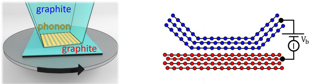
Figure 4.15 Schematics of the QTM junction (left), illustrating the formation of a continuously twistable interface between two graphite flakes. A bias voltage V_b is applied across the junction, and the conductance G is measured (right). A significant tunneling contribution arises from inelastic phonon scattering processes at the interface. Adapted from [92].
