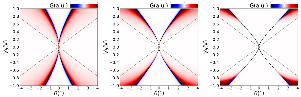
(a) d_g = 0.5nm , ( C_g = 566 \frac{nF}{cm^2} ). (b) d_g = 1.5nm , ( C_g = 189 \frac{nF}{cm^2} ). (c) d_g = 4.0nm , ( C_g = 71 \frac{nF}{cm^2} ). Figure 4.37 Dependence on hBN thickness (Capacitance). The gray (black) line corresponds to the onset (nesting).
