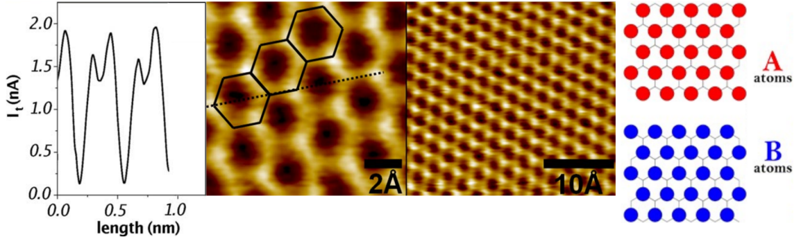
Figure 4.3 STM image (middle), line profile along the dashed lines (left) of Graphite at constant-height and V_b = -300mV . Illustration of monomer (A) and non-monomer (B) sites (right). Adapted from [84].
