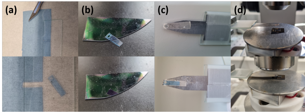
Figure 3.28 Preparation of the transfer slide: (a) A window is cut into a piece of adhesive tape. (b) Polymer layer with flake centered in the window is peeled of the substrate. (c) Flake is aligned with the hole on the transfer slide. (d) Transfer slide is mounted on the transfer stage and brought into contact with the cantilever.
