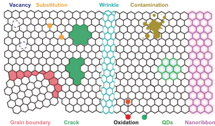
Figure 4.6 Schematic of Structural Disorder in Graphene. Adapted from [85].
