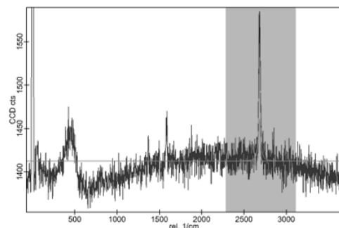
Figure 3.29 Raman spectrum of MLG with 2D-peak situated in grey area
