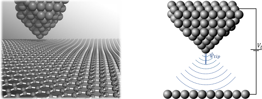
Figure 4.2 STM Working Principle. Adapted from [82].
