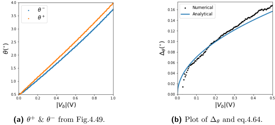
Figure 4.61 Asymmetry between the nesting lines.
