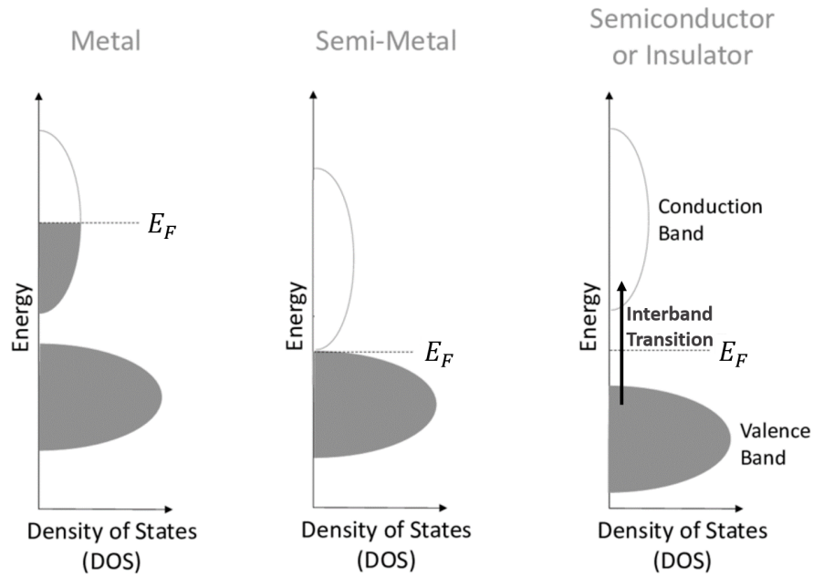
Figure 2.9 Electronic Structure of Solids. Adapted from [25].
