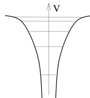
Figure 2.11 Potential V . Adapted from [16].
