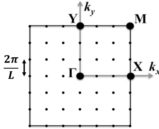
Figure 2.5 Brillouin zone of a square lattice with high symmetry points \Gamma , M , and X . Adapted from [18].
