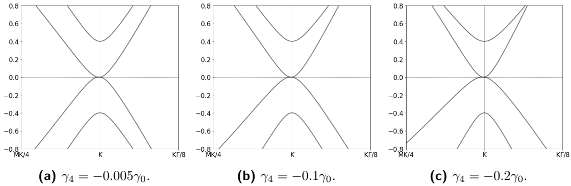
Figure 2.36 Band structure plots showing the effects of varying \gamma_4 .
