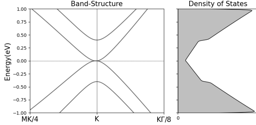
(a) Band structure and DOS.
