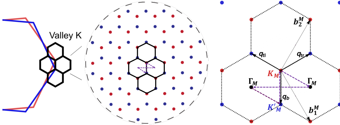
Figure 2.50 Emergence of the moiré Brillouin zone in the extended zone scheme from the momentum mismatch in the \mathbf{K} -valley. The purple dashed path marks the trajectory in \mathbf{k} -space for Fig.2.55, Fig.2.57, and Fig.2.58. Adapted from [34][51].
