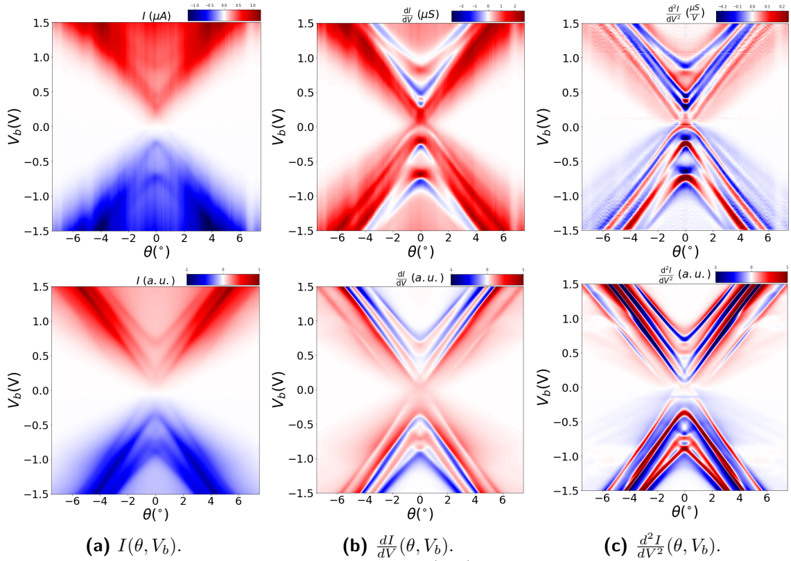
Figure 4.73 Measured tunneling spectra (top) and the corresponding theoretical calculations (bottom).
