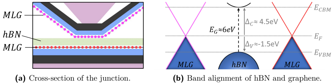
Figure 4.19 hBN as a tunneling barrier. Adapted from [14].
