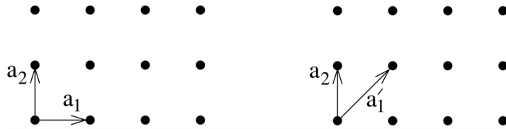
Figure 2.2 Illustration of two different sets of basis vectors generating the same square lattice. Adapted from [16].
