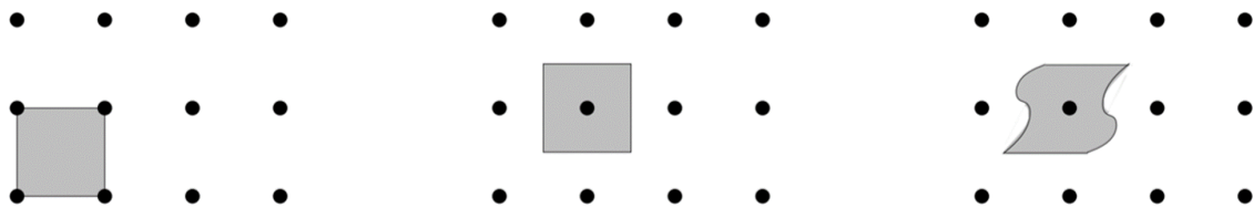
Figure 2.3 Different choices of primitive unit cells. Adapted from [16].
