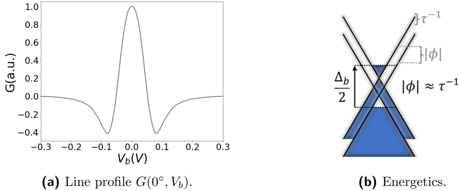
Figure 4.40 Broadening in the Conductance near charge neutrality.
