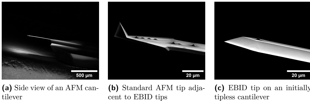
Figure 3.13 Tips fabricated by EBID on AFM cantilevers.
