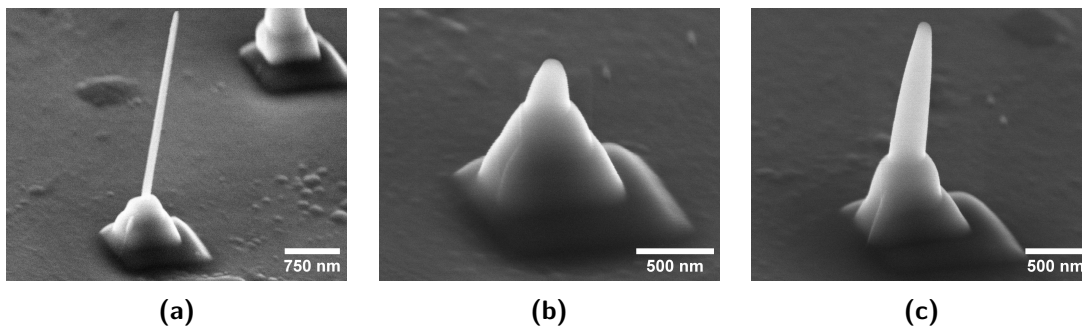
Figure 3.15 EBID-Pillars. The parameters are altered in accordance to Tab.3.1.
