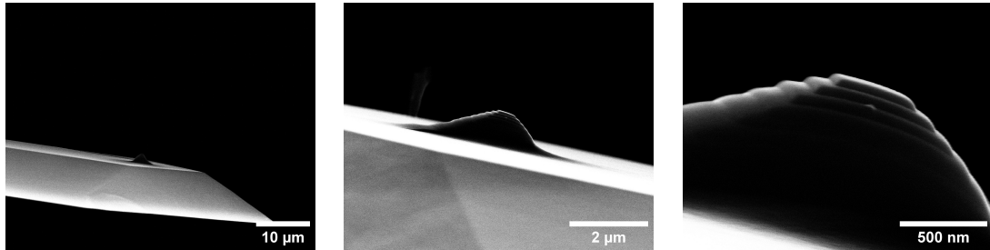
Figure 3.23 EBID-tip on cantilever, showcasing substantial improvement upon increasing the aperture size.
