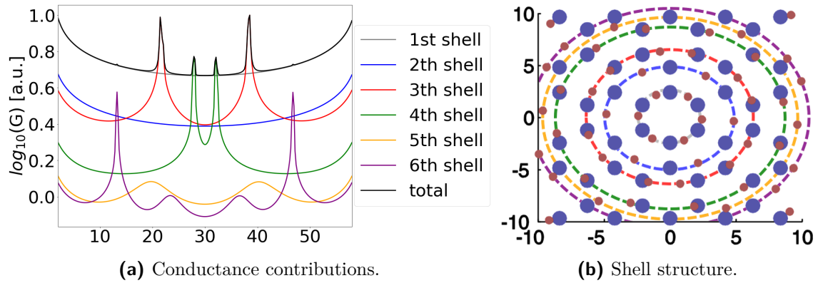
Figure 4.14 Shell numbering of the momentum lattice and the calculation of respective contributions from each shell.
