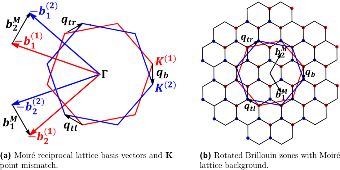
Figure 2.43 Moiré reciprocal lattice. Adapted from [41].
