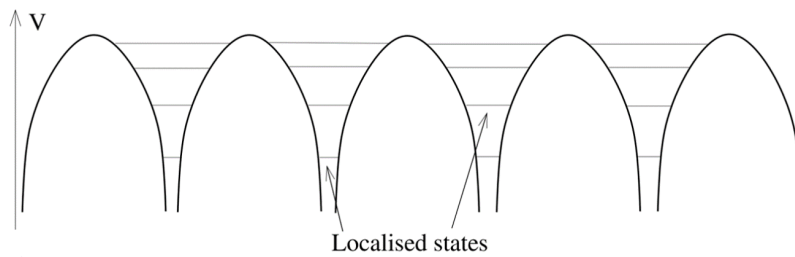
Figure 2.13 Crystal lattice potential composed of several atomic potentials. Adapted from [16].
