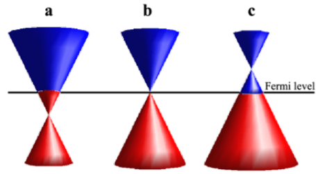
Figure 4.65 Fermi-level for n-type (a), neutral (b) and p-type (c) doping. Adapted from [101].
