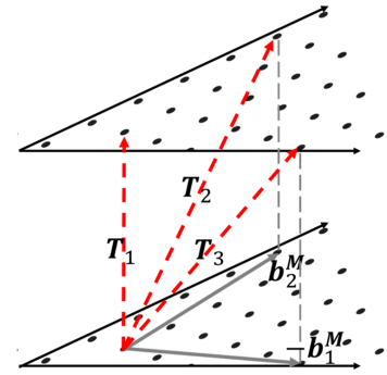
Figure 4.33 Tunneling in the Reduced Zone Scheme.
