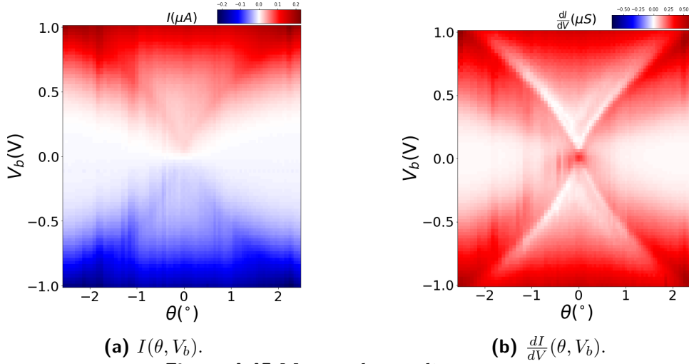
Figure 4.45 Measured tunneling spectra.
