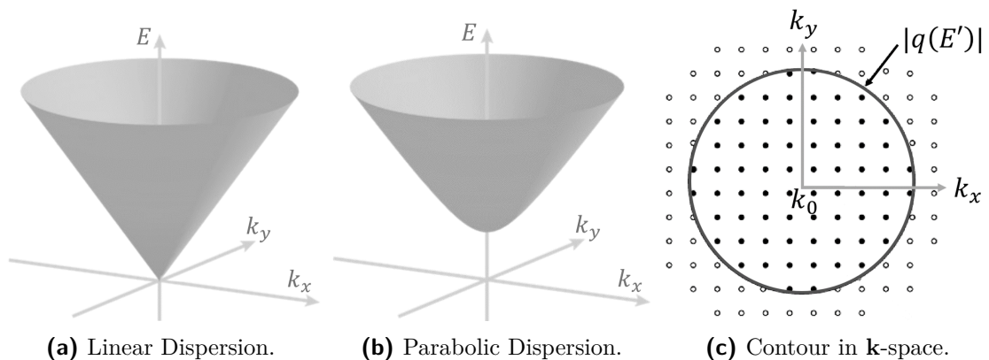
Figure 2.8 Illustrations of typical dispersion relations in E - \mathbf{k} -space. Adapted from [24].
