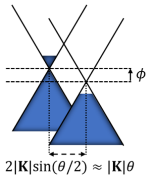
Figure 4.27 E- \mathbf{k} -space geometry.
