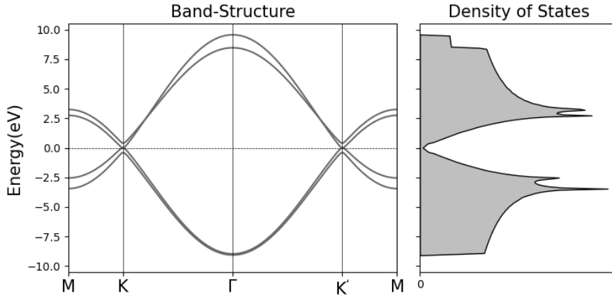
Figure 2.29 Band structure and DOS calculated using the tight-binding method.
