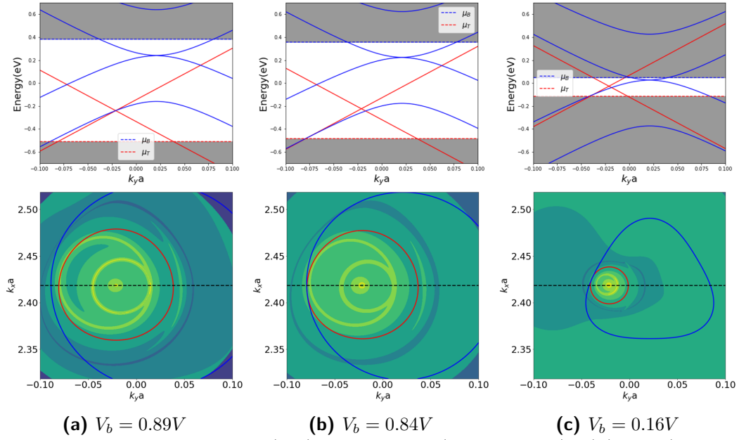
Figure 4.53 Energy bands (top) along \mathbf{k} -path (dashed black), I(\mathbf{k}) map (bottom) centered at \mathbf{K}_D (unrotated), showing the energy contours of MLG (red) and BLG (blue) at \mu_T . Background brightness is proportional to the logarithmic current.
