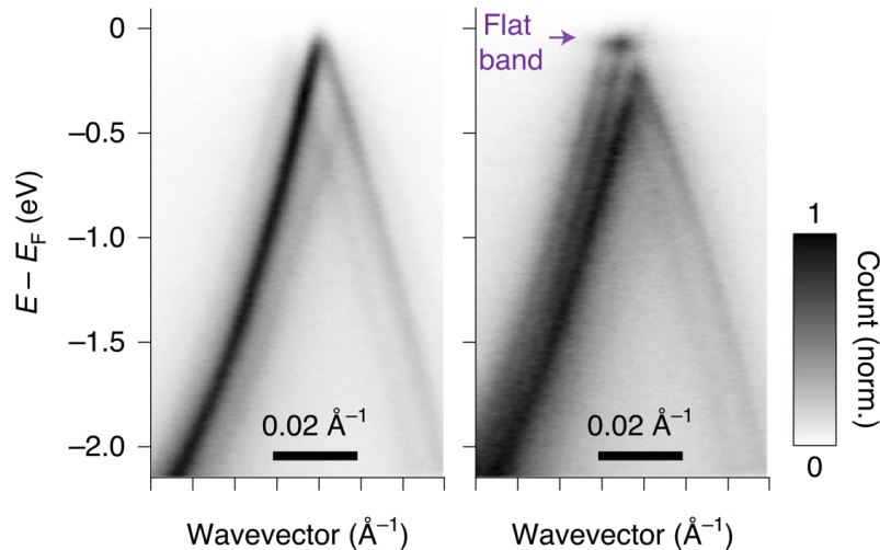
Figure 1.5 ARPES spectrum of graphene (left) and TBG (right). Adapted from [12].
