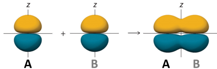
Figure 2.20 Bonding configuration within a diatomic unit cell. Adapted from [27].
