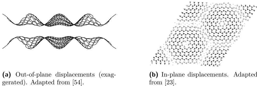
Figure 2.56 Effects of lattice relaxation on the crystal structure.
