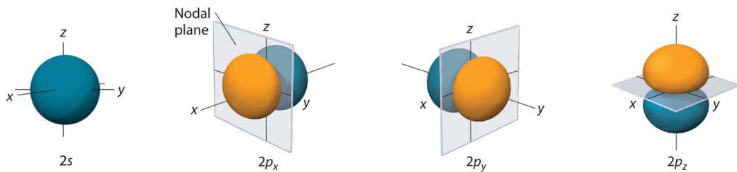
Figure 2.12 Orbital Shapes of the Second Shell. Adapted from [27].
