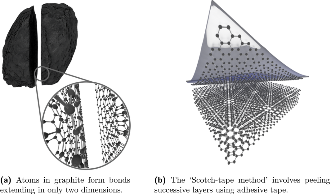
Figure 1.1 Mechanical exfoliation of graphene from bulk graphite. Adapted from [2].
