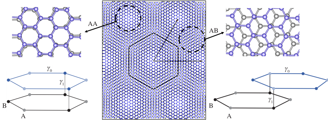
Figure 2.40 Moiré pattern resulting from alternating regions of AA and AB stacking. Adapted from [30][42][43].
