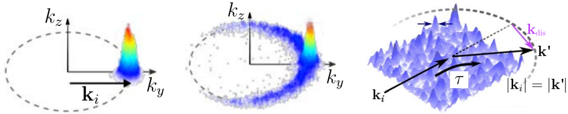
(a) Initial Wave Packet. (b) Scattered Wave Packet. (c) |\mathbf{k}_i\rangle scatters after mean time \tau .
