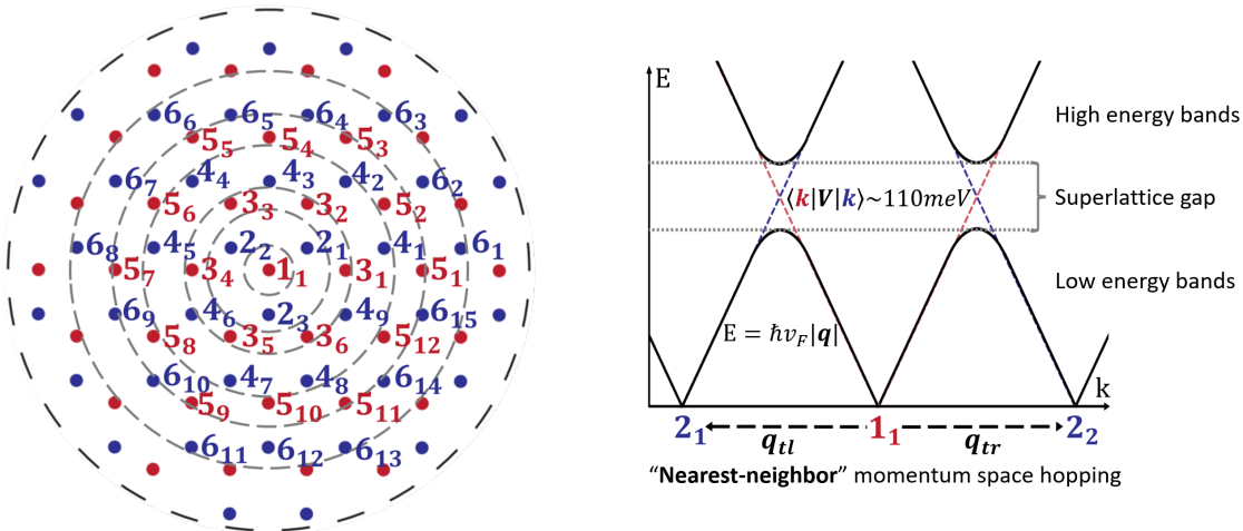
Figure 2.51 Shell numbering and next-nearest-neighbor interaction in the momentum lattice.
