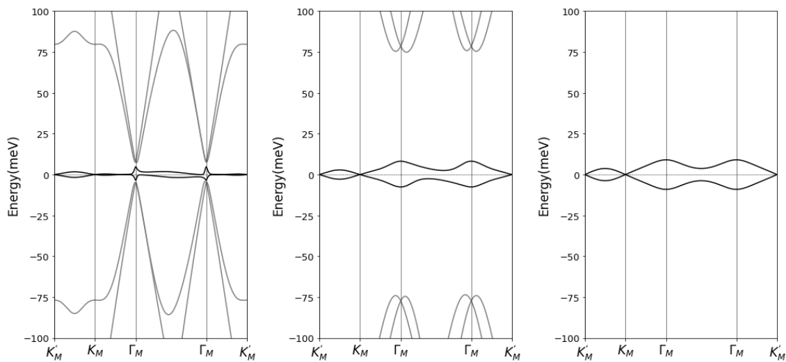
Figure 2.57 Effect of lattice relaxation (from left to right: \omega = 1.0, 0.5, 0.0 ) on the band structure of TBG plotted along the path in Fig.2.50 for \theta = 1.05^\circ .
