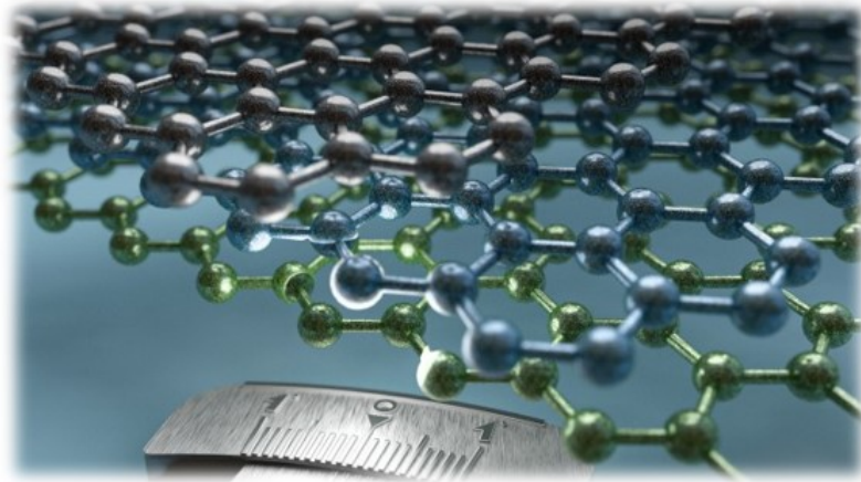
Figure 1.3 Illustration of the rotational misalignment between graphene layers. Adapted from [5].
