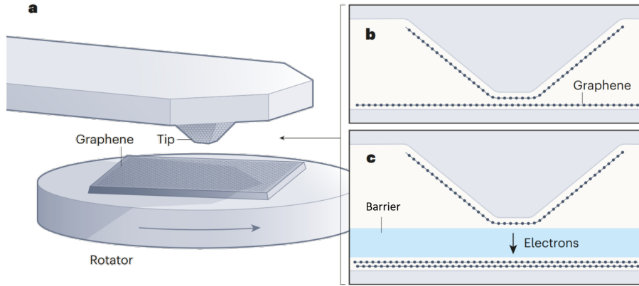
Figure 1.6 a The quantum twisting microscope, which can be used to control the angular alignment between one or more sheets comprising single layers of atoms, such as graphene. The microscope consists of a pyramid-shaped tip that is covered in one sheet (of graphene, for example), and brought into contact with a second sample on a rotator. b In this way, the microscope can be used to control the angular alignment of such layers in situ. c The device can also measure and change the way in which the energy of electrons in the multilayered structure depends on their momentum. In this mode, the electrons move through an added barrier layer of an insulating material. Adapted from [13].
