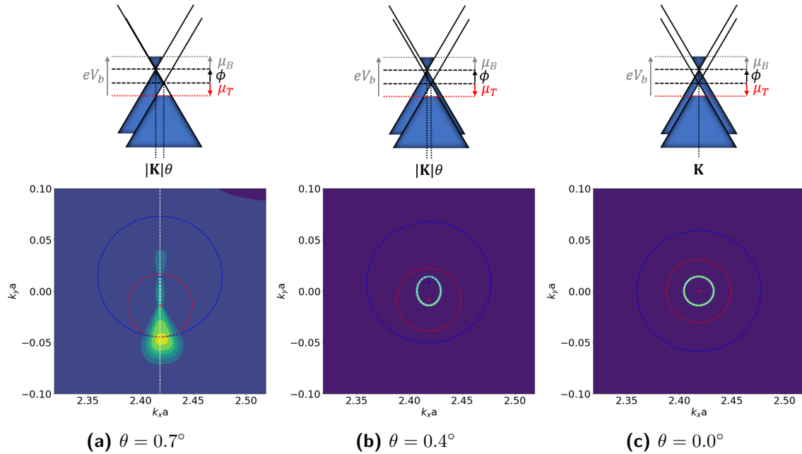
Figure 4.32 Energetics (above) and I(\mathbf{k}) -map (below) centered at \mathbf{K}_D (unrotated) for V_b = 0.4 V. White lines correspond to intersection lines, blue and red lines represent energy contours of band states at \mu_T (rotated by \pm\theta/2 respectively). Background brightness is proportional to current strength.
