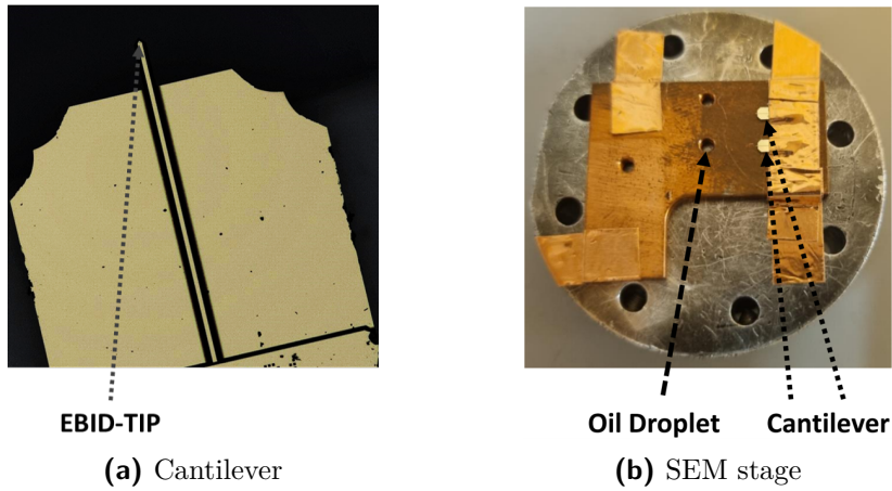
Figure 3.14 Sample preparation process.
