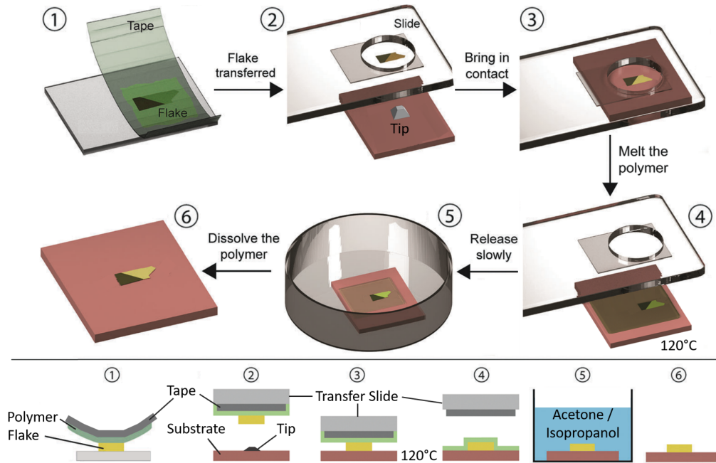
Figure 3.30 Polymer membrane transfer technique: The target flake is exfoliated onto a layer of PPC, which is used to pick up the flake with an adhesive tape (1). The tape is attached to a transfer slide and the flake aligned with the tip on the substrate (2). The flake is brought into contact with the substrate (3). The substrate is heated to 120°C, melting the polymer layer (4). The remaining polymer residues are then dissolved in acetone and isopropanol (5), leaving the flake transferred onto the tip (6). Adapted from [79]
