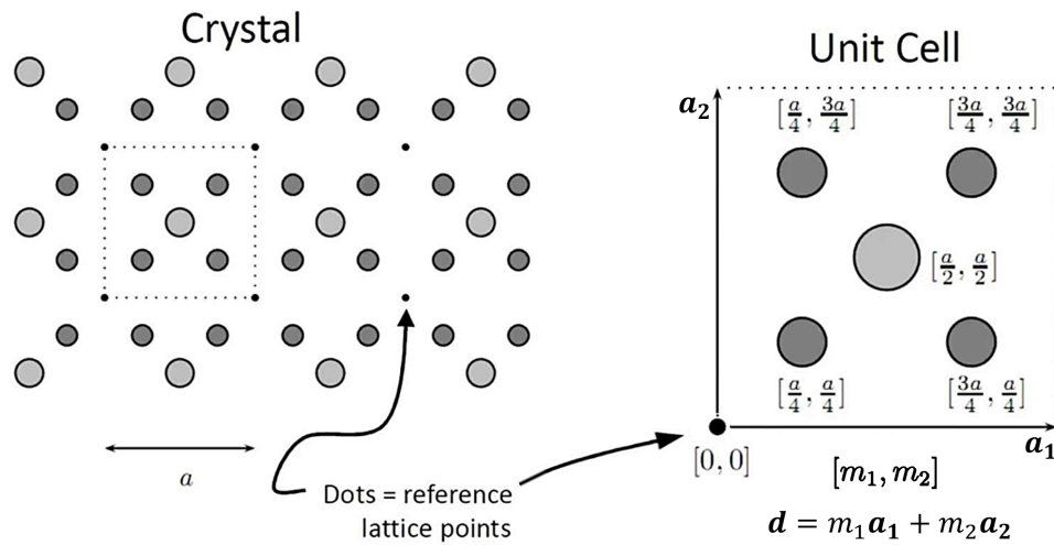
Figure 2.4 Inner structure of a unit cell, where [m_1, m_2] are the relative positions of the atomic constituents in terms of the basis vectors. Adapted from [17].
