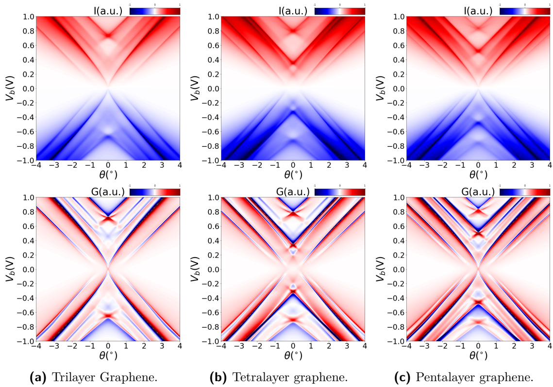
Figure 4.69 Tunneling spectra without barrier interaction.
