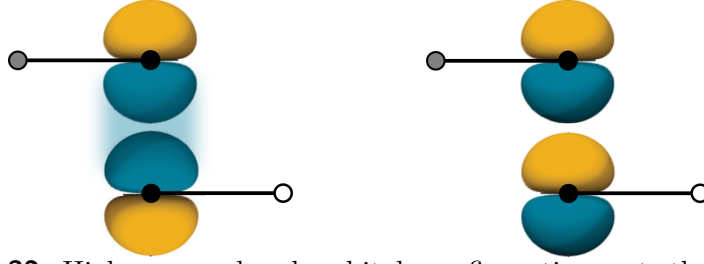
Figure 2.32 High-energy band orbital configurations at the \mathbf{K} -point. Adapted from [27].
