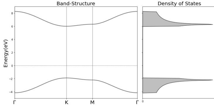
Figure 4.18 Band structure and DOS calculated using the tight-binding method.
