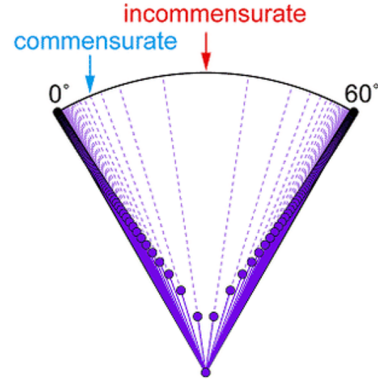
(b) \theta -distribution for forming commensurate TBG. The corresponding Moiré period is represented by the length of solid line (with logarithmic scale).
