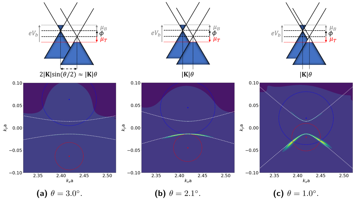
Figure 4.31 Energetics (above) and I(\mathbf{k}) -map (below) centered at \mathbf{K}_D (unrotated) for V_b = 0.4\text{ V} . White lines correspond to intersection lines, blue and red lines represent energy contours of band states at \mu_T (rotated by \pm\theta/2 respectively). Background brightness is proportional to current strength.
