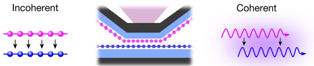
Figure 5.1 Illustrations of incoherent and coherent tunneling across the 2D junction. In incoherent tunneling, electrons tunnel at various locations independently, with the tunneling rate being proportional only to the local wavefunction squared. In coherent tunneling, however, trajectories interfere, making the tunneling sensitive to the phase variations of the wavefunctions in both the top and bottom layers across the junction. Adapted from [14].
