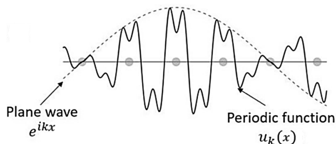
Figure 2.6 Bloch wave, consisting of a periodic function modulated by a plane wave. Adapted from [20].
