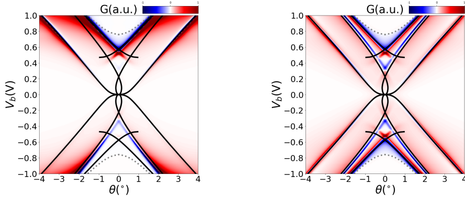
(a) With barrier interaction (b) Without barrier interaction Figure 4.51 Tunneling spectra with nesting (solid black) and matching (dashed gray) lines.
