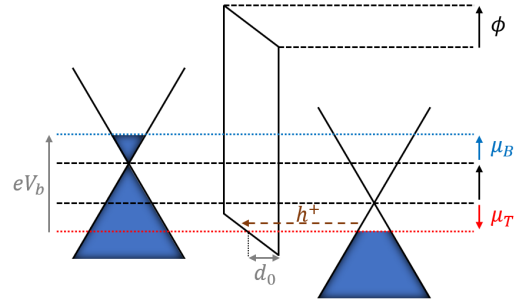
Figure 4.25 Tunneling between hBN and graphene.
