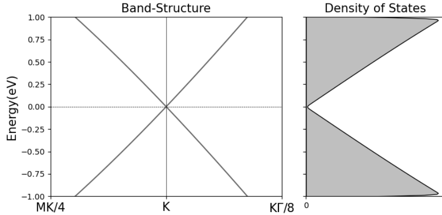
Figure 2.26 Low energy band structure and DOS calculated using the tight-binding method.
