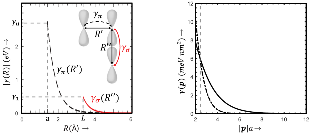
(a) Decay of the real space amplitude of 2.109(black dashed line) and 2.110(red solid line)
