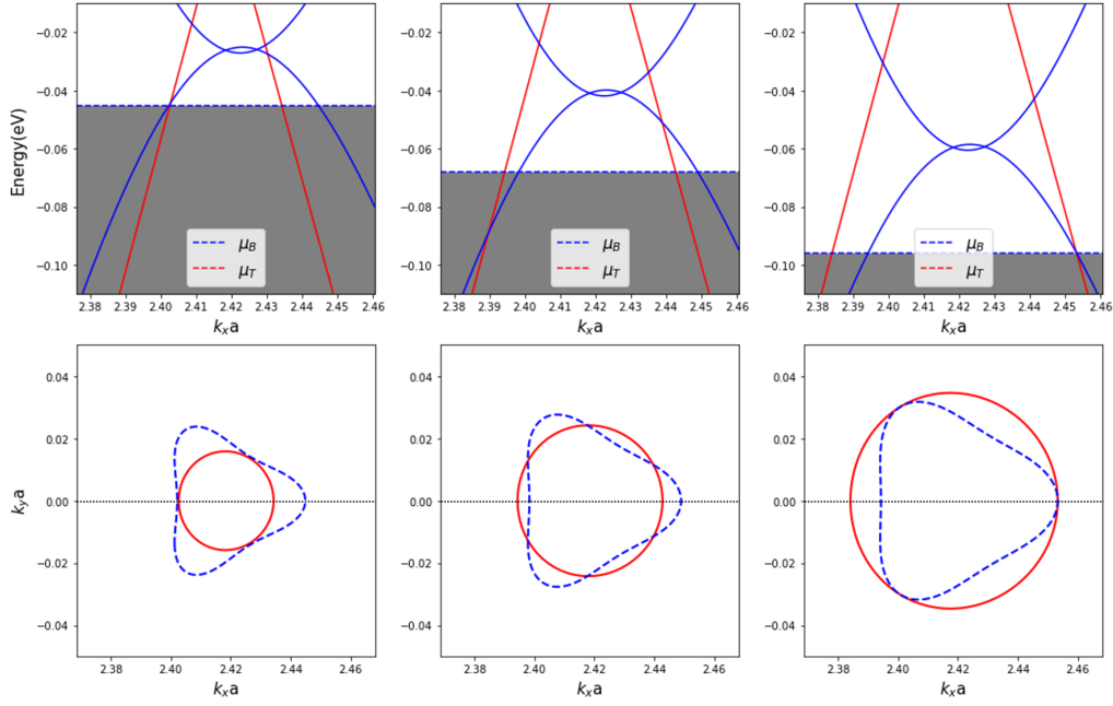
Figure 4.58 Energy bands (top) and Fermi surface of MLG (solid red) and empty band states (dashed blue) of BLG in \mathbf{k} -space at \mu_B . The Fermi surface is depicted for bias voltages of V_b = -0.17V (left), V_b = -0.23V (middle), and V_b = -0.29V (right).
