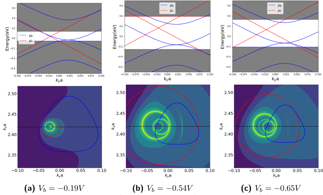
Figure 4.54 Energy bands (top) along \mathbf{k} -path (dashed black), I(\mathbf{k}) map (bottom) centered at \mathbf{K}_D (unrotated), showing the energy contours of MLG (red) and BLG (blue) at \mu_T (left) and \mu_B (middle and right). Background brightness is proportional to the logarithmic current.
