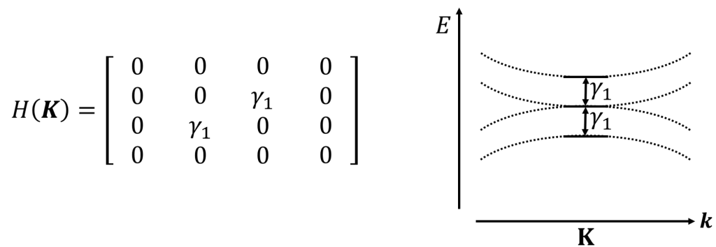
Figure 2.31 Energy bands at the \mathbf{K} -point.
