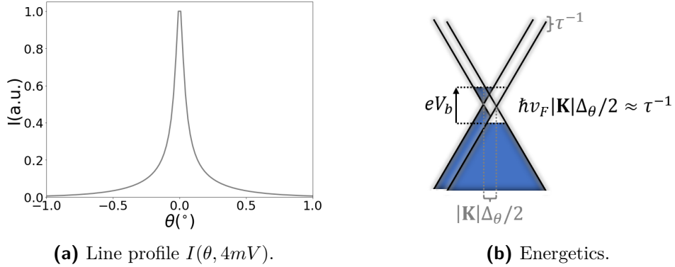
Figure 4.39 Lorentzian current broadening near charge neutrality.
