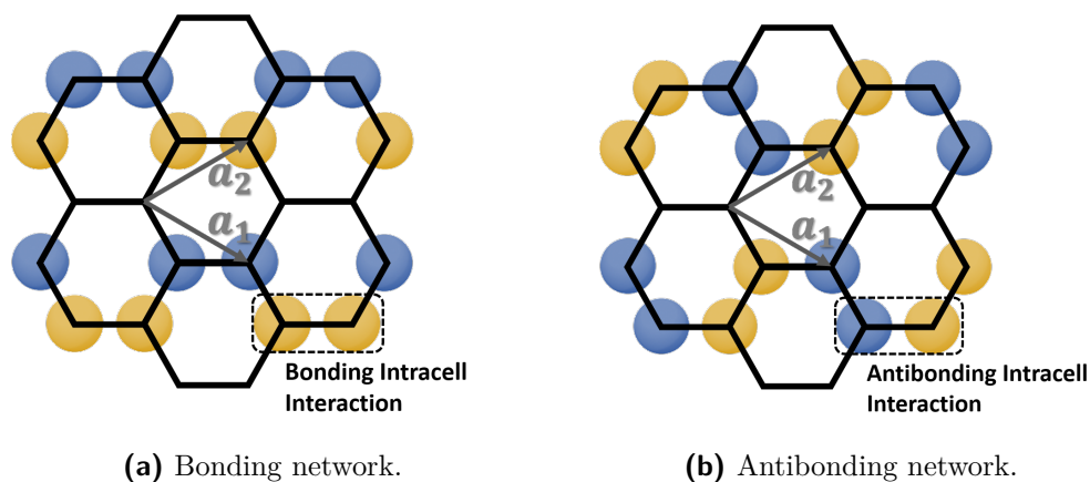
Figure 2.24 Bonding and antibonding orbital networks at the \mathbf{K} -point.
