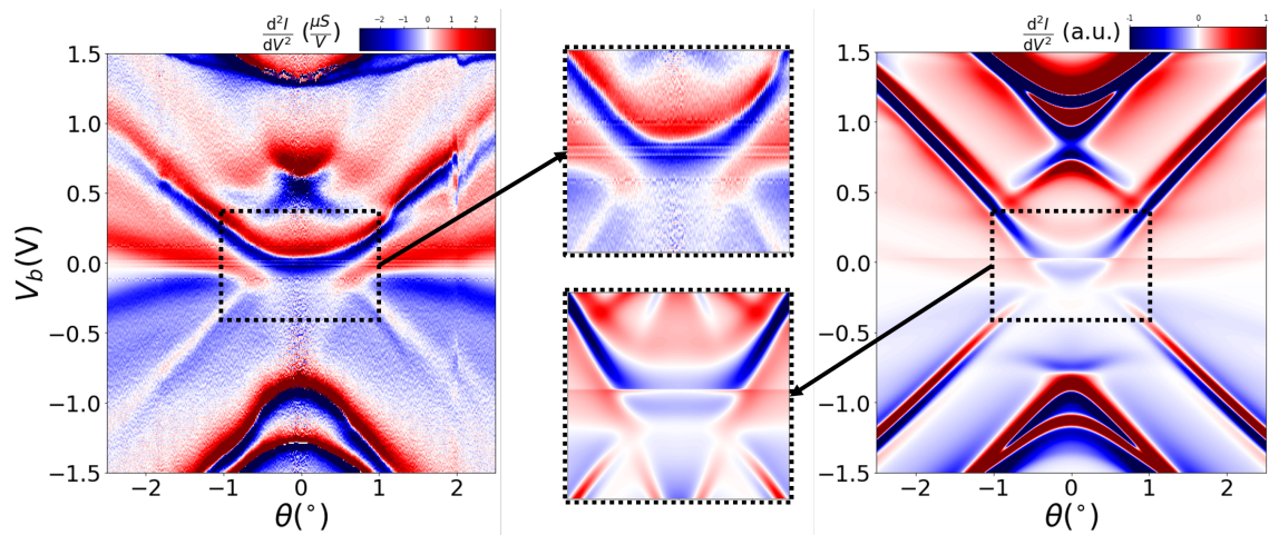
Figure 4.68 Measurement (left) and numerical calculation (right), with C_g = 5.66 \frac{\mu F}{cm^2} , including MLG strained by 0.8% and doped by \Delta\mu_T = +0.15eV .
