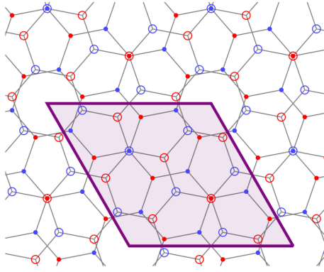
(a) Unit cell (purple rhombus) at commensurate angle \theta_0 \approx 38.2^\circ . The top (bottom) atoms are represented by dots (circles) and the A (B) sublattices in each layer are colored blue (red).
