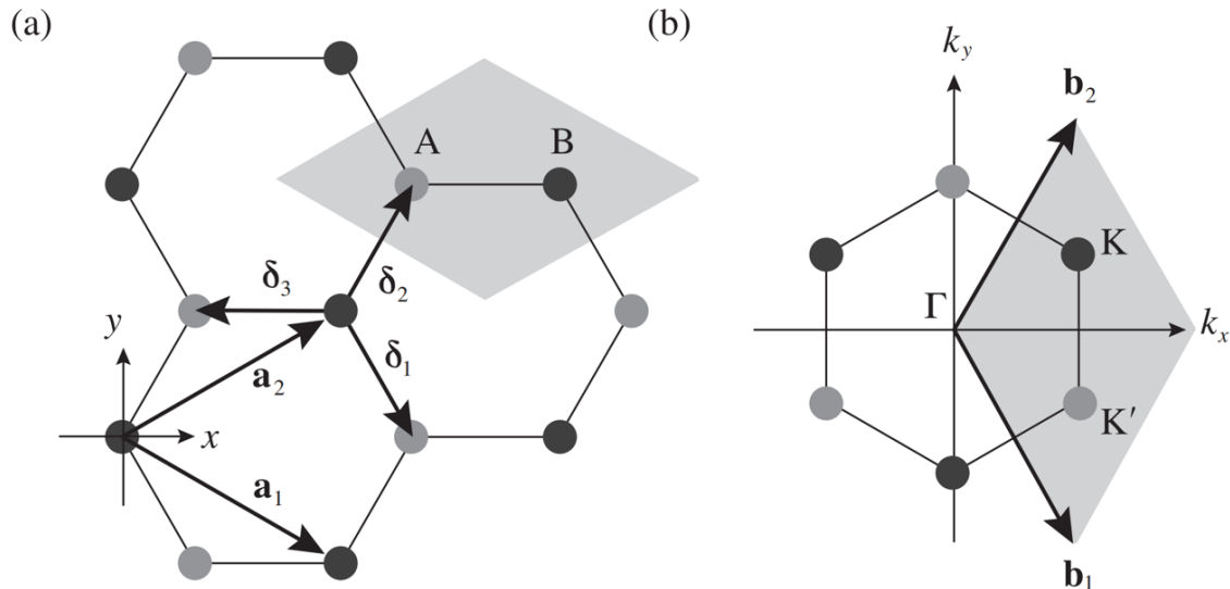
Figure 2.17 (a) Real-space honeycomb graphene lattice. The lattice consists of two overlapping Bravais sublattices, A (gray dots) and B (black dots). The primitive unit cell is drawn as a shaded area. \mathbf{a}_1 and \mathbf{a}_2 are the primitive lattice vectors. \delta_1 , \delta_2 , and \delta_3 are vectors pointing from a B atom to its nearest A atoms. (b) Reciprocal unit cell of graphene drawn as a shaded area. \mathbf{b}_1 and \mathbf{b}_2 are the primitive vectors of the reciprocal lattice. Dirac points \mathbf{K} (black dots) and \mathbf{K}' (gray dots) are marked. Adapted from [30].
