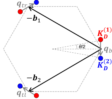
Figure 2.49 k-space geometry.
