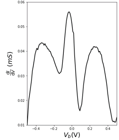
Figure 4.78 Measured line profile \frac{dI}{dV}(0^\circ, V_b) .
