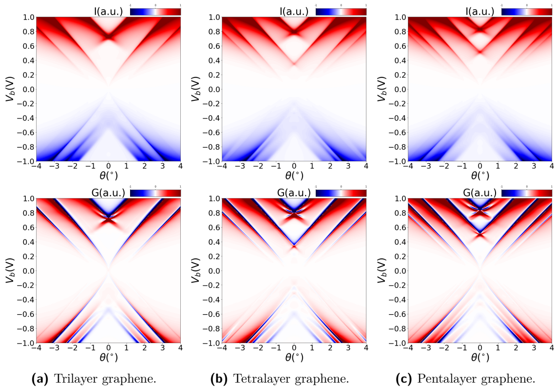
Figure 4.70 Tunneling spectra including barrier interaction.
