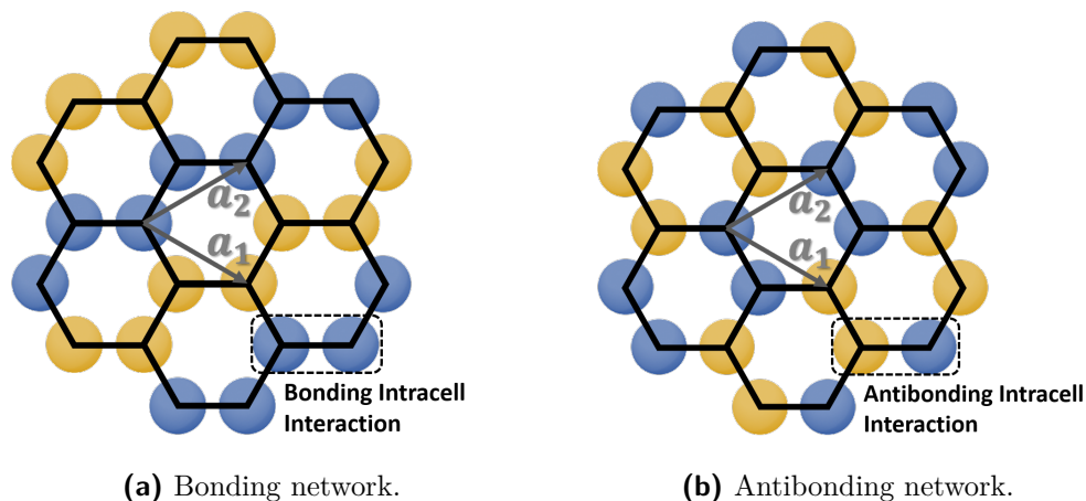
Figure 2.23 Bonding and antibonding orbital networks at the \mathbf{M} -point.
