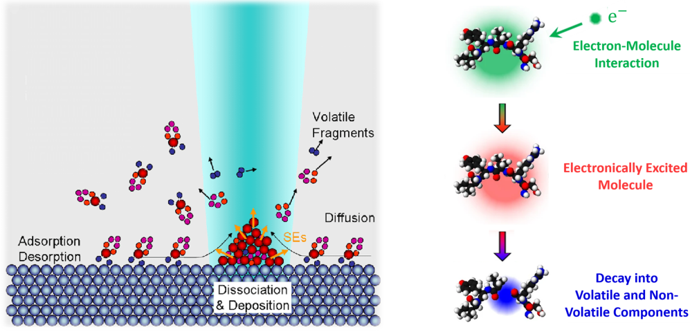
Figure 3.11 Electron-beam induced dissociation and deposition. Adapted from [66].
