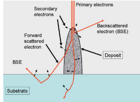
Figure 3.16 Deposition events on the surface of the deposit. Adapted from [75].
