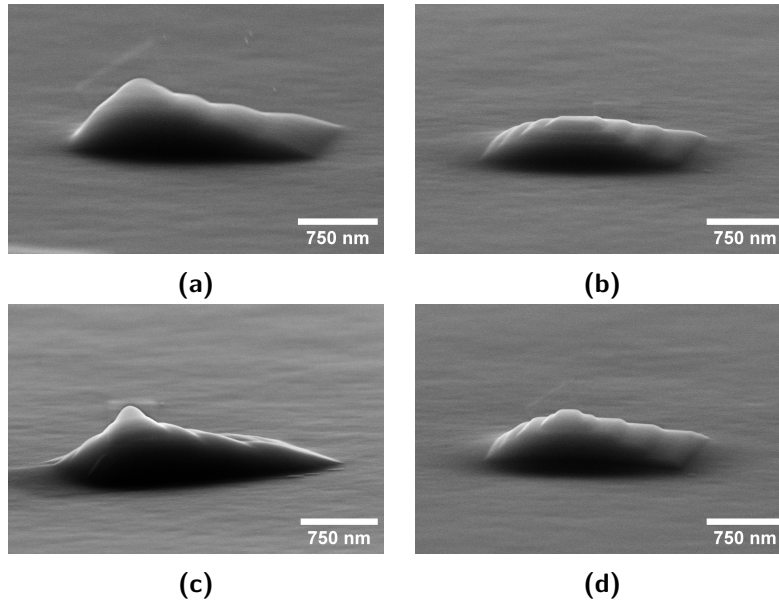
Figure 3.19 EBID-pyramids. The parameters are altered in accordance to Tab.3.2.
