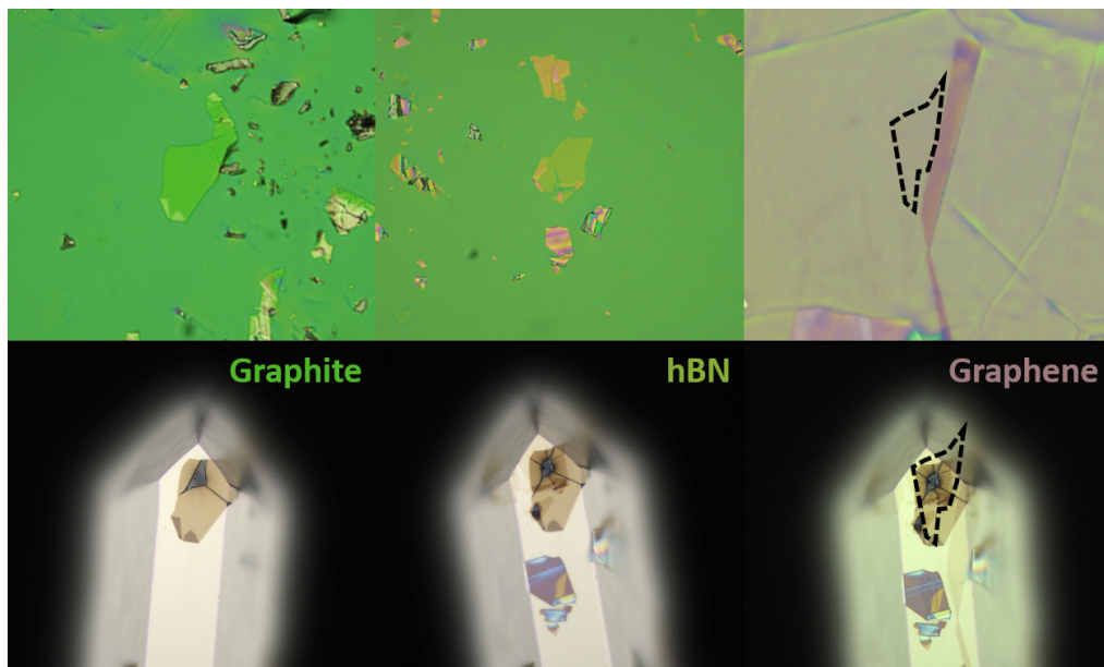
Figure 3.31 Successive transfer of graphite, hBN and graphene: Exfoliated flakes on coated Si/SiO 2 substrate (top). Flakes after transfer on cantilever (bottom).
