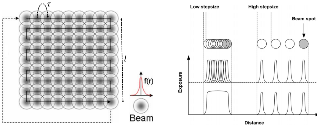
Figure 3.17 Digital serpentine raster scan scheme with overlap (left) and corresponding energy deposition (right). The Gaussian beam dwells for a time \tau and is then moved by one object pixel ( px ) to the next exposure spot. After completing one raster scan ( frame ), the beam repeats the pattern. Adapted from [66].
