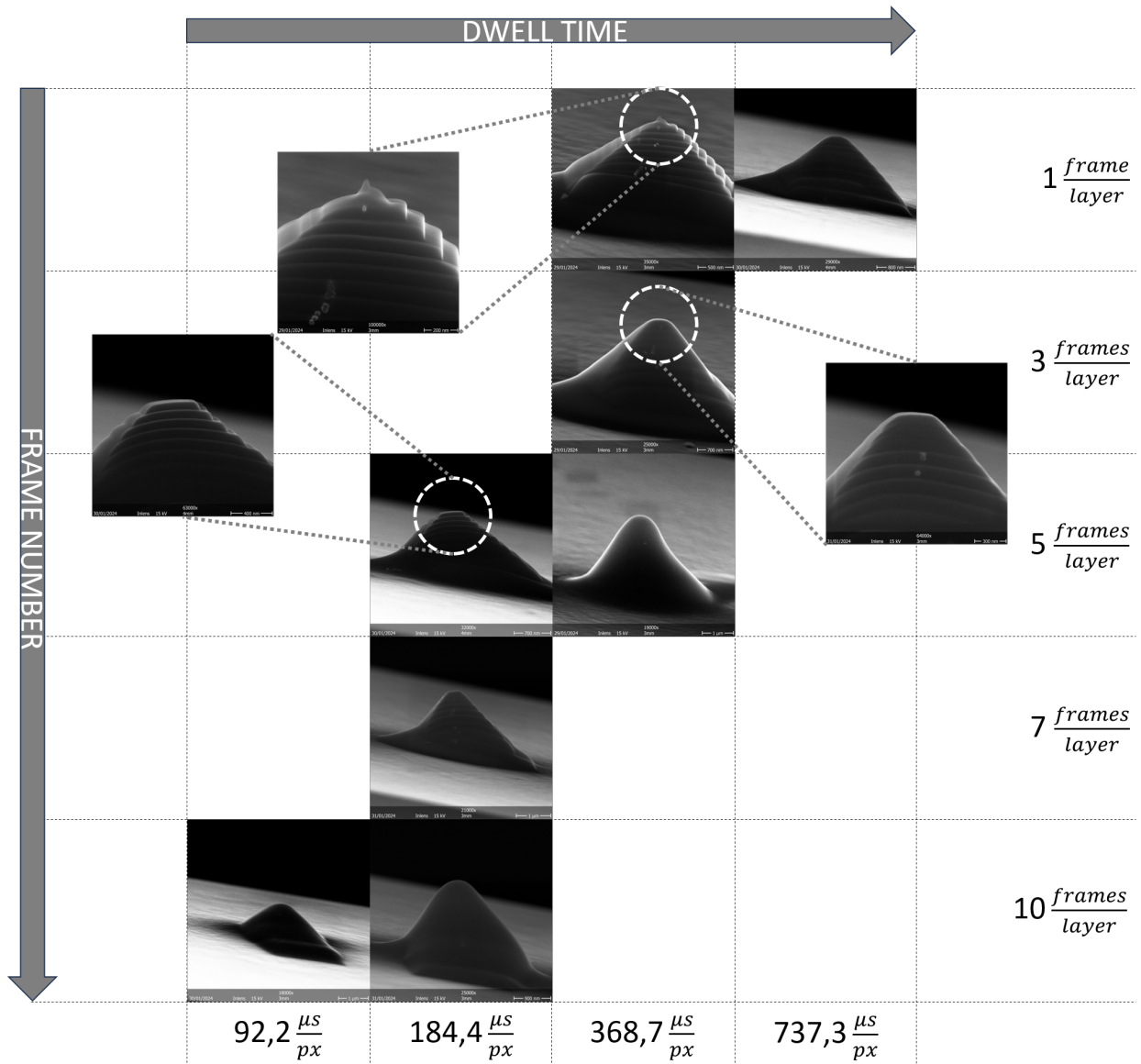
Figure 3.25 Dependence of pyramid growth on dwell time and frame number for the EBID process at U = 15kV , D = 60\mu m , M = 50000 , with the layer structure as shown in Fig.3.24.
