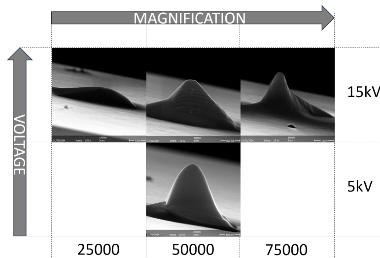
Figure 3.26 Dependence of pyramid growth on magnification and acceleration voltage for the EBID process at D = 60\mu m , \tau = 368.7\frac{\mu s}{px} , with the layer structure as in Fig.3.24, and 3 frames per layer.
