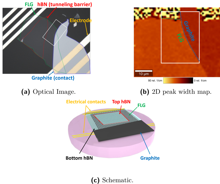
Figure 3.36 Sample device: (a)&(c) The stack consists of hBN (spacer towards substrate), graphite (contact for FLG), FLG (system to probe), thin hBN (insulating barrier). (b) Raman map of the white rectangle in (a): Boundary between the area where graphite lies below the FLG flake, causing the broadening of the 2D-peak. Adapted from [14].
