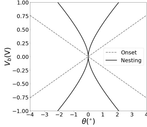
Figure 4.36 Schematic of the charge-neutral MLG-MLG tunneling experiment, showing the analytically derived lines in the \theta - V_b plane, which correspond to the momentum-resolved 'onset' and 'nesting' conditions.
