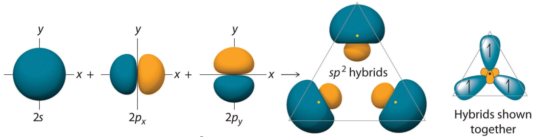
Figure 2.14 sp^2 -hybrid orbitals. Adapted from [27].
