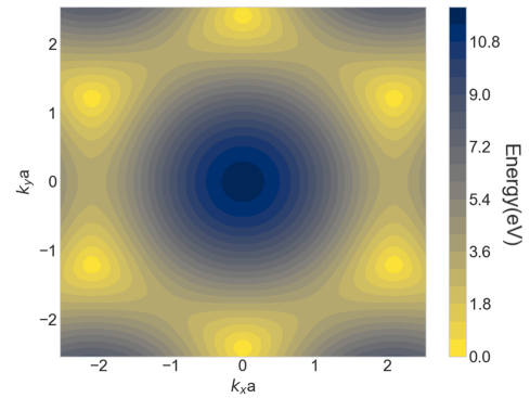
(c) Contour plot of the conduction band.
