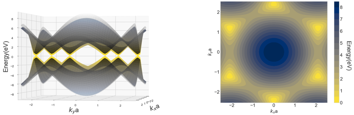
Figure 2.30 Energy surface plot and contour plot of the conduction band in BLG.
