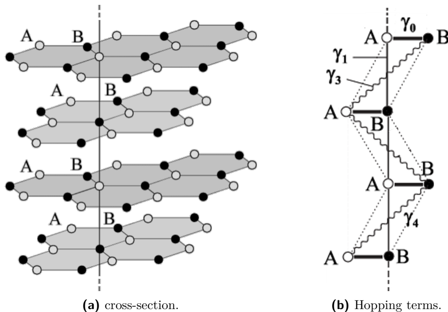
Figure 2.37 Crystal structure of FLG. Adapted from [37].
