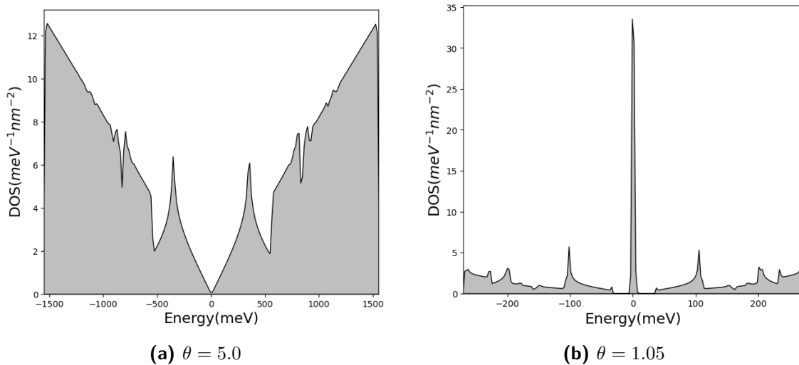
Figure 2.61 DOS of TBG.
