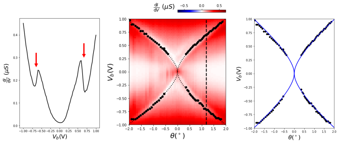
(a) Nesting features (b) \frac{dI}{dV} and nesting features (c) Fit of eq.4.36
