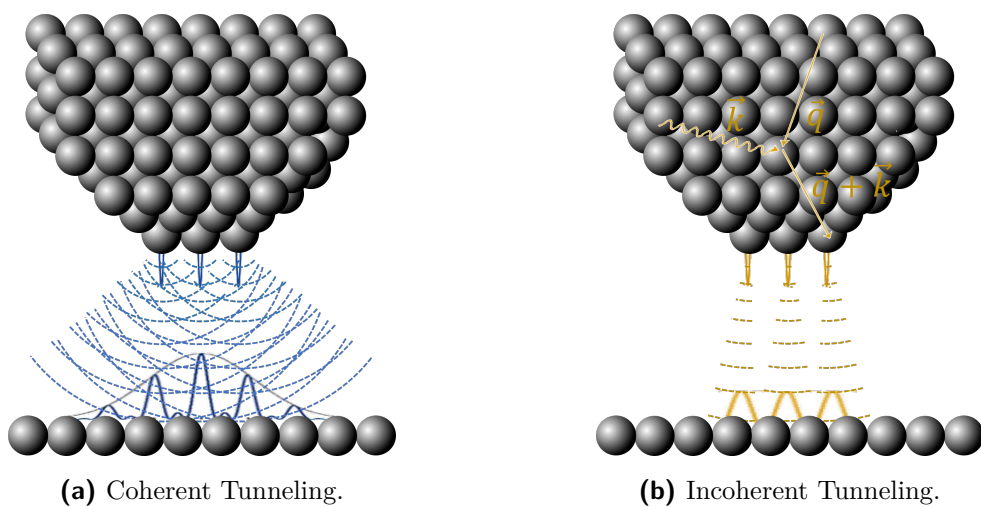
Figure 4.4 Phase (in-)coherent Tips.
