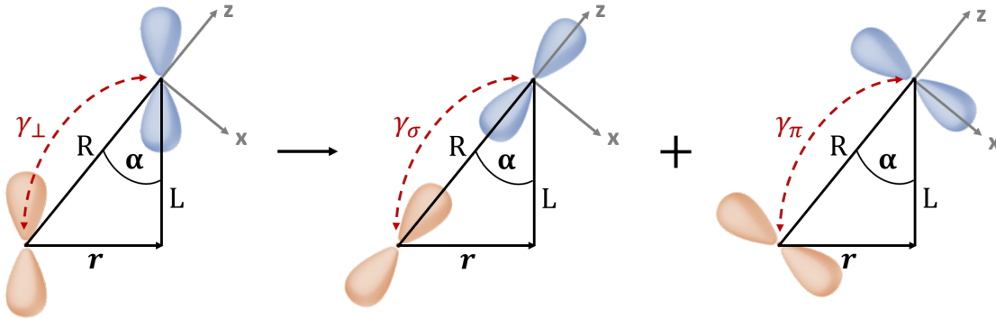
Figure 2.46 Illustration of the overlap integral calculation: One p_z -orbital is initially located at the origin, while another p_z -orbital is at the separation vector \mathbf{R} . The coordinate system is rotated so that the second orbital shifts to R\hat{\mathbf{z}} , resulting in the orbitals becoming linear combinations of p_x and p_z .
