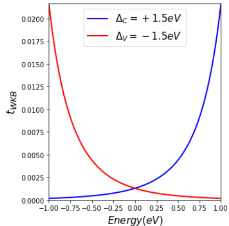
Figure 4.56 WKB amplitudes for different barrier configurations.
