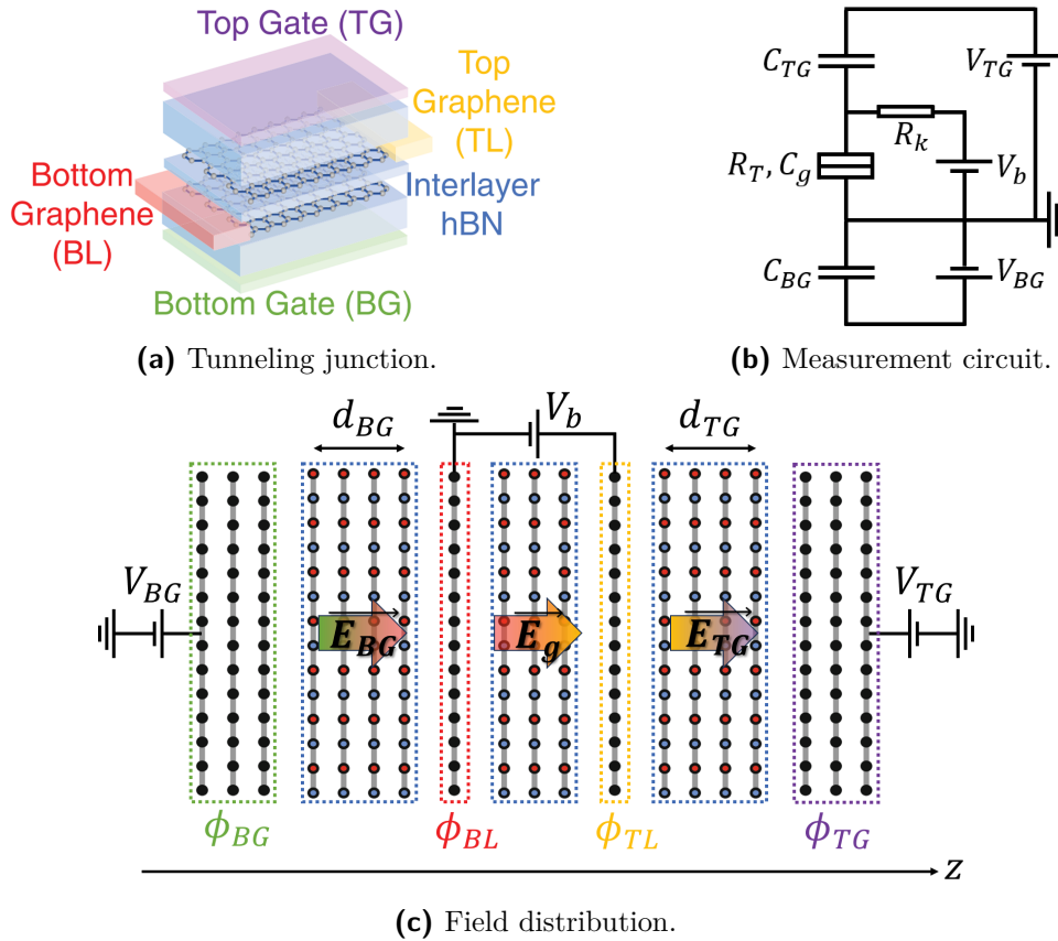
Figure 4.22 Electrostatics of the tunnel junction. Adapted from [96].
