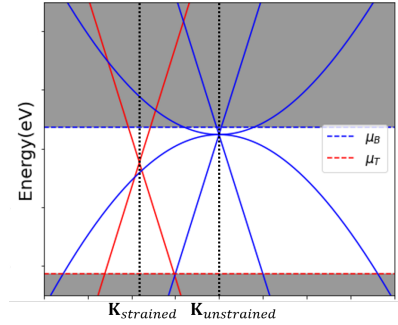
Figure 4.74 Tunneling between linear band onsets at finite bias.
