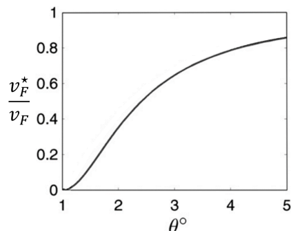
Figure 2.59 Renormalized Dirac-point band velocity. Adapted from [6].
