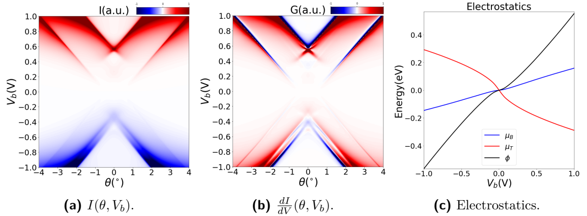
Figure 4.49 Simulated tunneling spectra for BLG.
