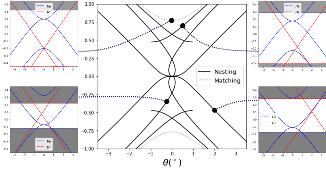
Figure 4.50 Nesting and matching lines in BLG (probed with MLG on tip).
