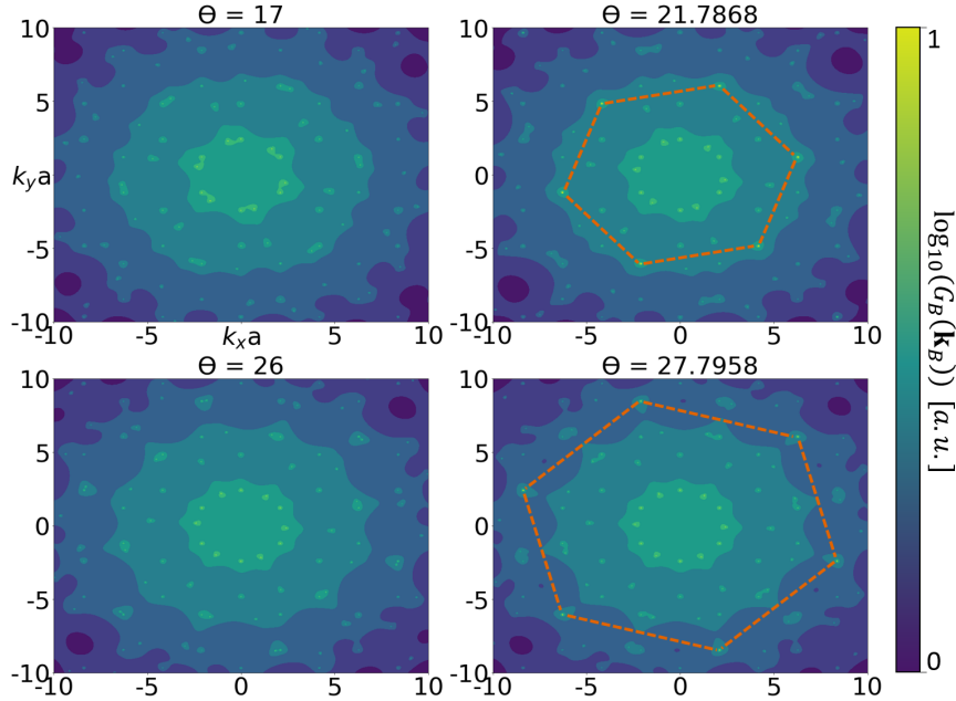
Figure 4.13 Mapping of conductance contribution \log_{10}(G_B(\mathbf{k}_B)) (eq.4.8) in an extended-zone scheme. Contribution strength is proportional to the brightness. Conductance contributions occur where the Fermi circles intersect and are significantly larger when the intersection occurs closer to the origin of momentum space. At commensurate angles, peaks arise in higher Brillouin zones.
