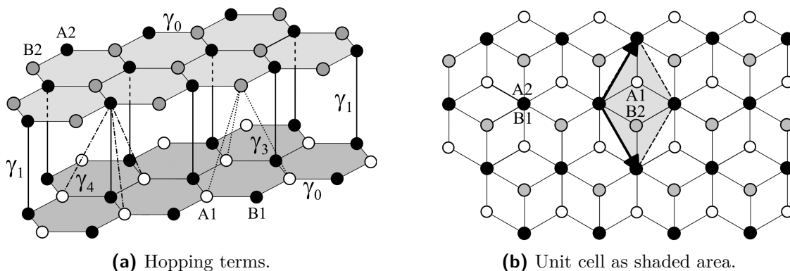
Figure 2.28 BLG lattice, consisting of four overlapping trigonal Bravais sublattices A_1, B_1, A_2 and B_2 . Adapted from [36].
