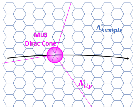
Figure 5.2 When the MLG probe layer is rotated relative to the sample system with a_{tip} \ll a_{sample} , its Dirac cone (pink circle) traces the energy bands along an arc (black) in momentum space.
