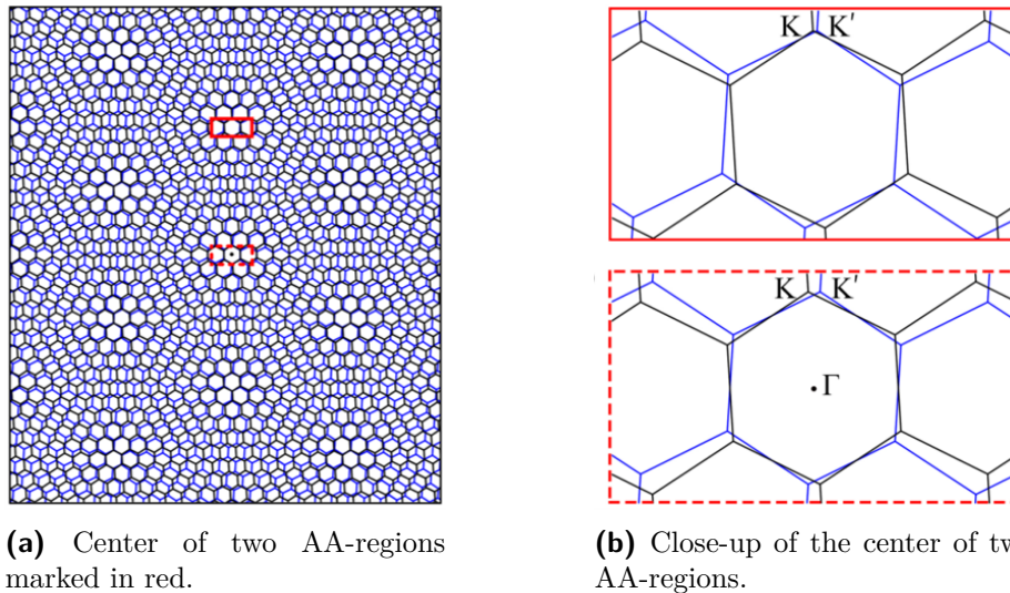
Figure 2.41 Primitive translations in the moiré lattice may not reproduce the same atomic configuration. Adapted from [43].
