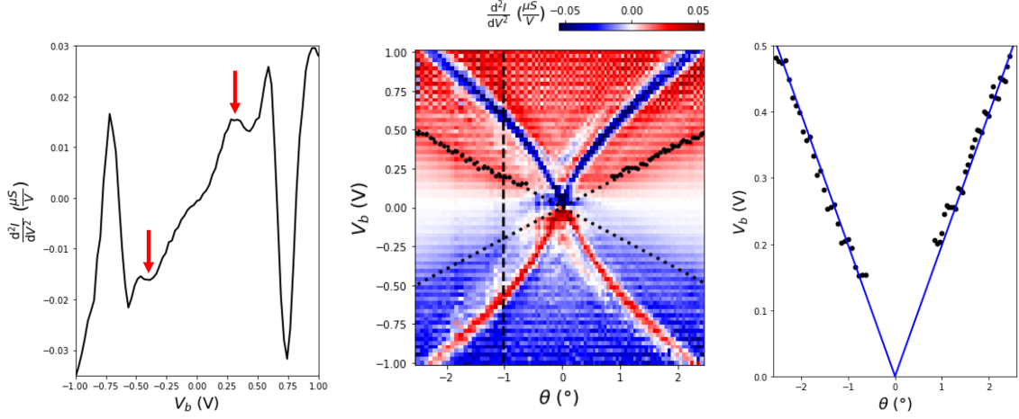
(a) Onset features. (b) \frac{d^2I}{dV^2} and onset features. (c) Fit of eq.4.35.
