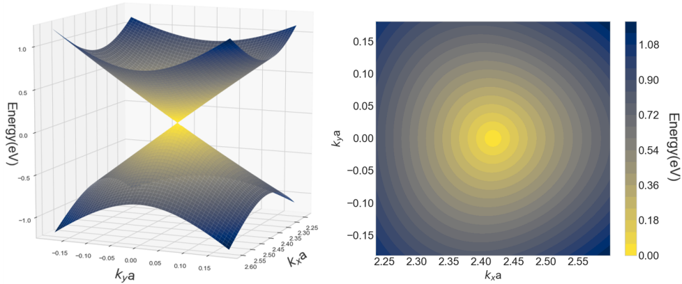
Figure 2.27 Low energy surface plot and contour plot of the conduction band.
