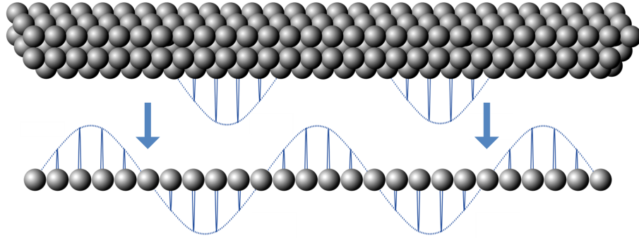
Figure 4.5 Interlayer Coupling of Bloch States.
