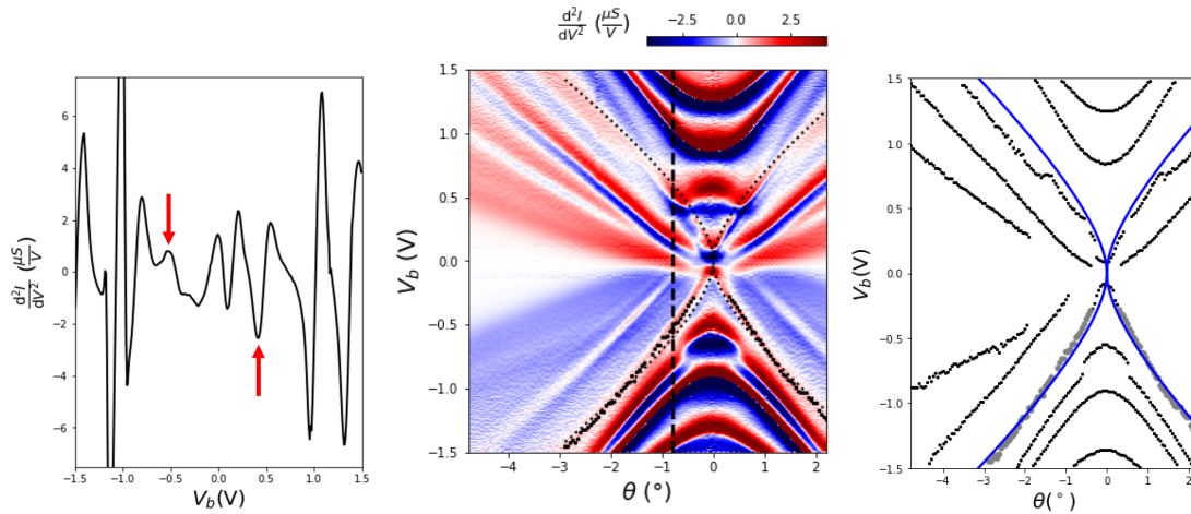
(a) Nesting features. (b) \frac{d^2I}{dV^2} and nesting features. (c) Fit of eq.4.70.
