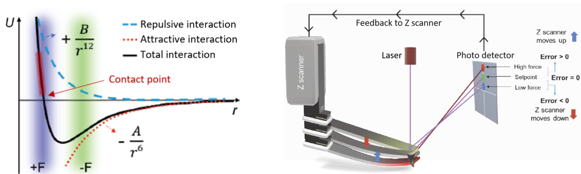
(a) Lennard-Jones Potential.
